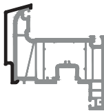
3312 260 gr/m Al cover cap sash
