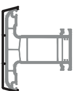
3316 416 gr/m Al cover cap mullion
