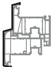
3319 507 gr/m Al cover cap sash-overhung
